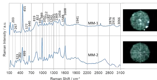
Fig. 3. The representative Raman spectra of the composite MM «Stahl 1018»
